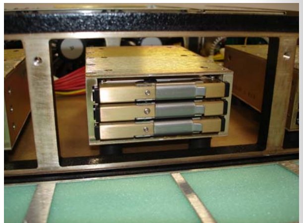
Detail of shock isolated Custom drive enclosure w/3 x 2.5" SATA drives
