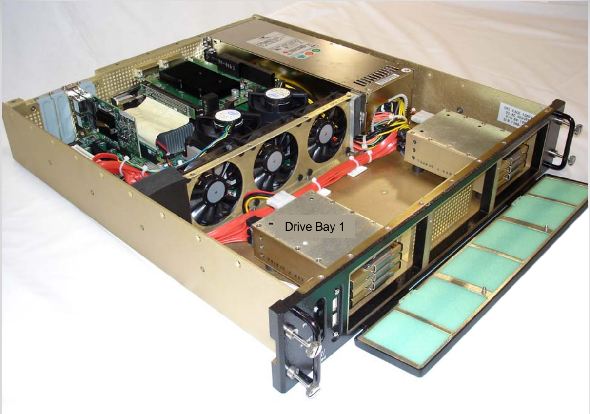
Shown with 2 of 3 3 x 2.5" drive bays mounted
